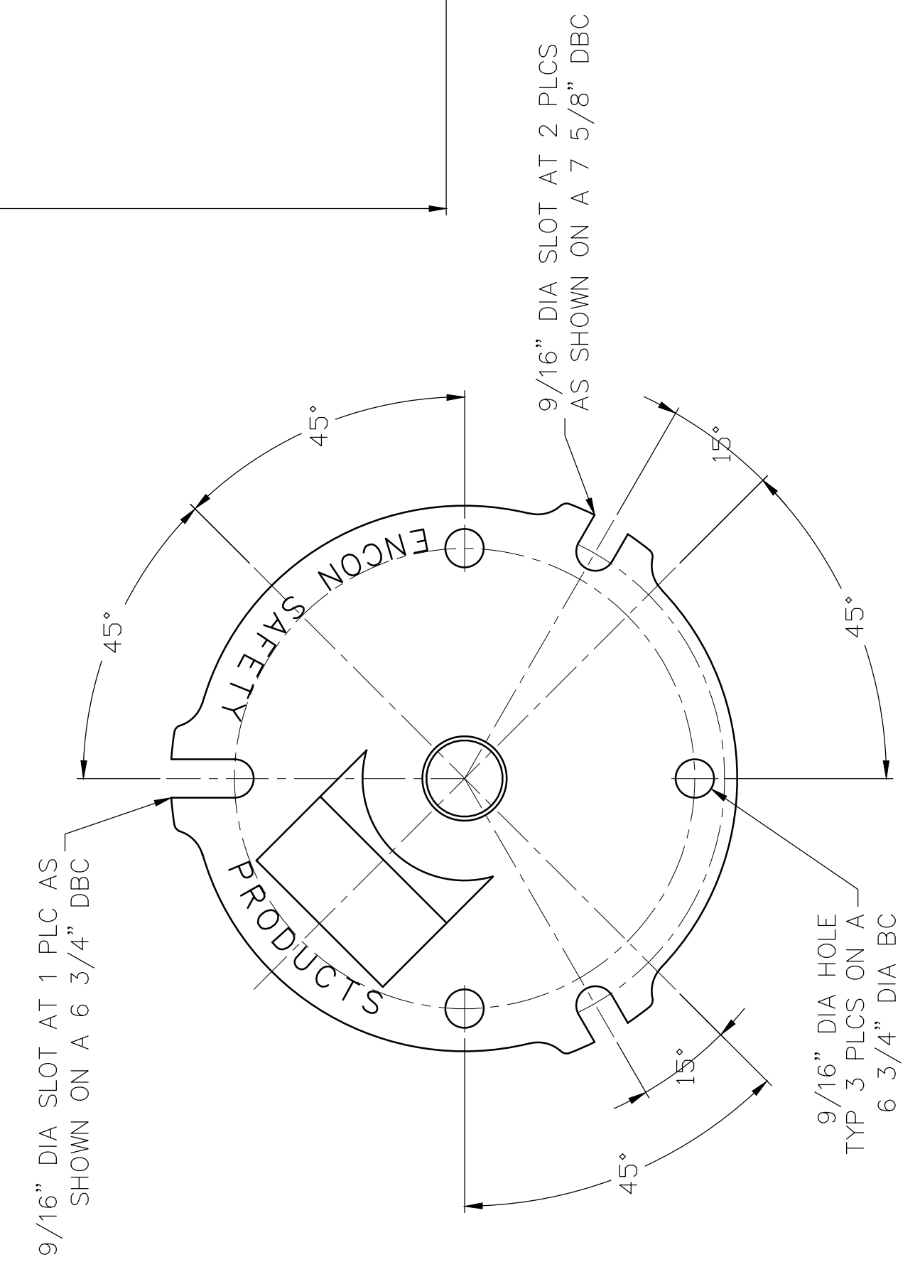
FLOOR FLANGE DETAIL SCALE: 1/2
