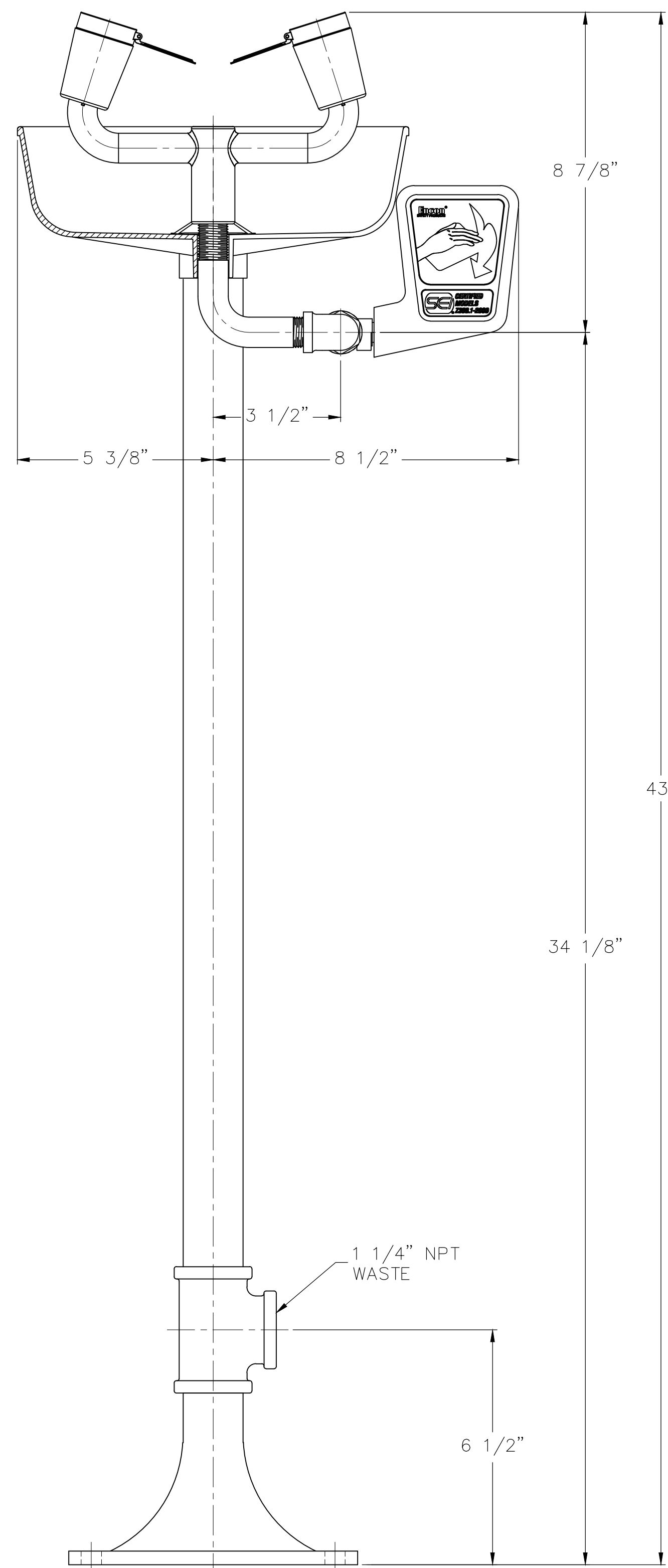
FRONT VIEW
